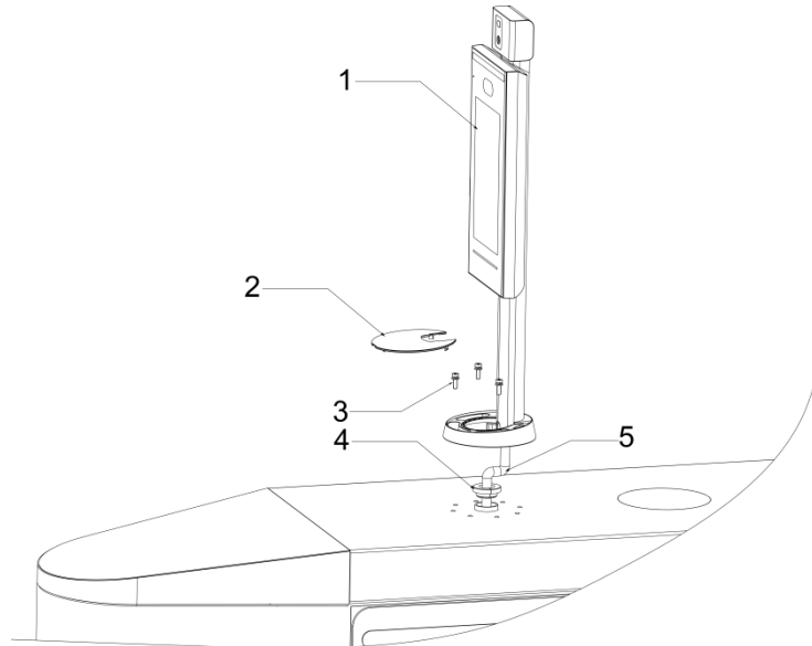
Figure 2-7 Applying silicon sealant to the terminal
