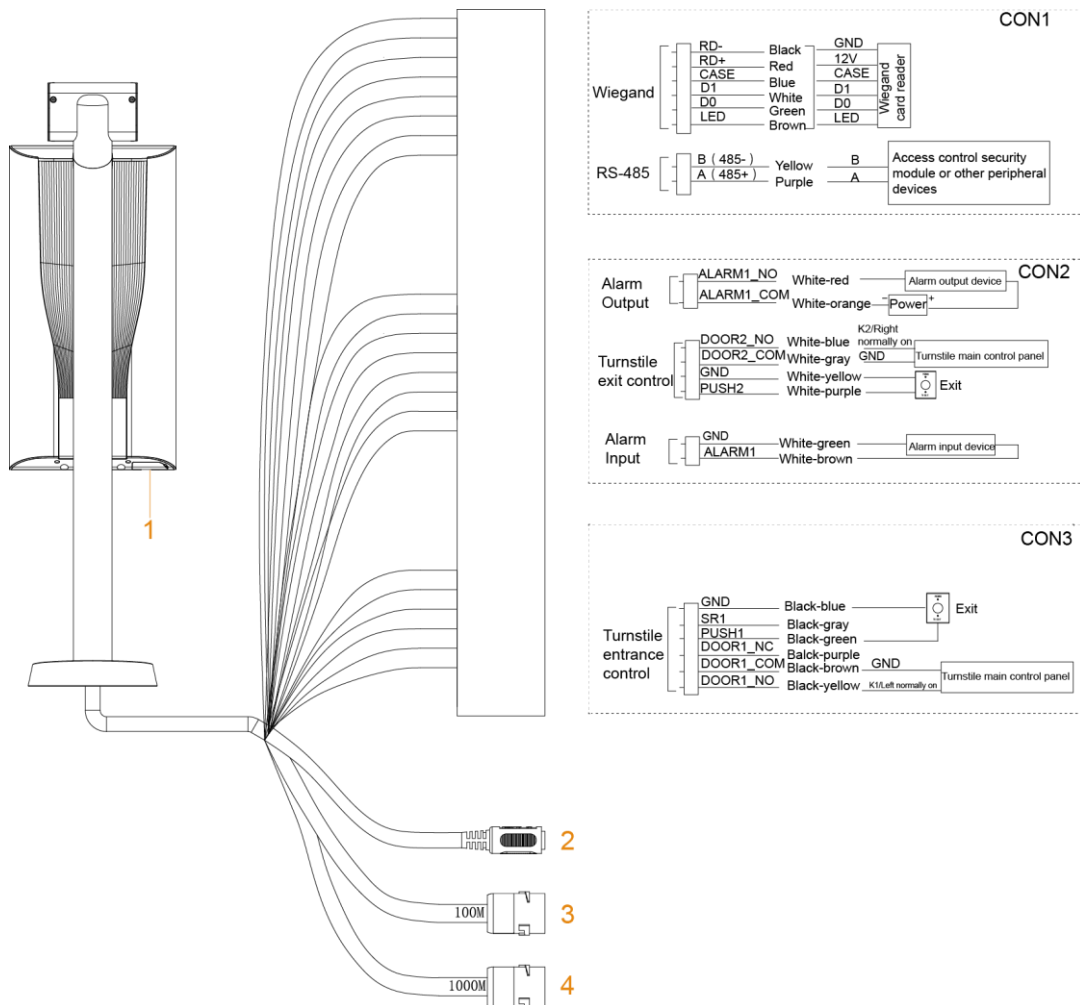
Figure 2-1 Cable connection
