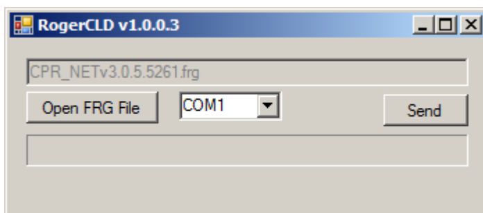
Rys. 13 Program RogerCLD
