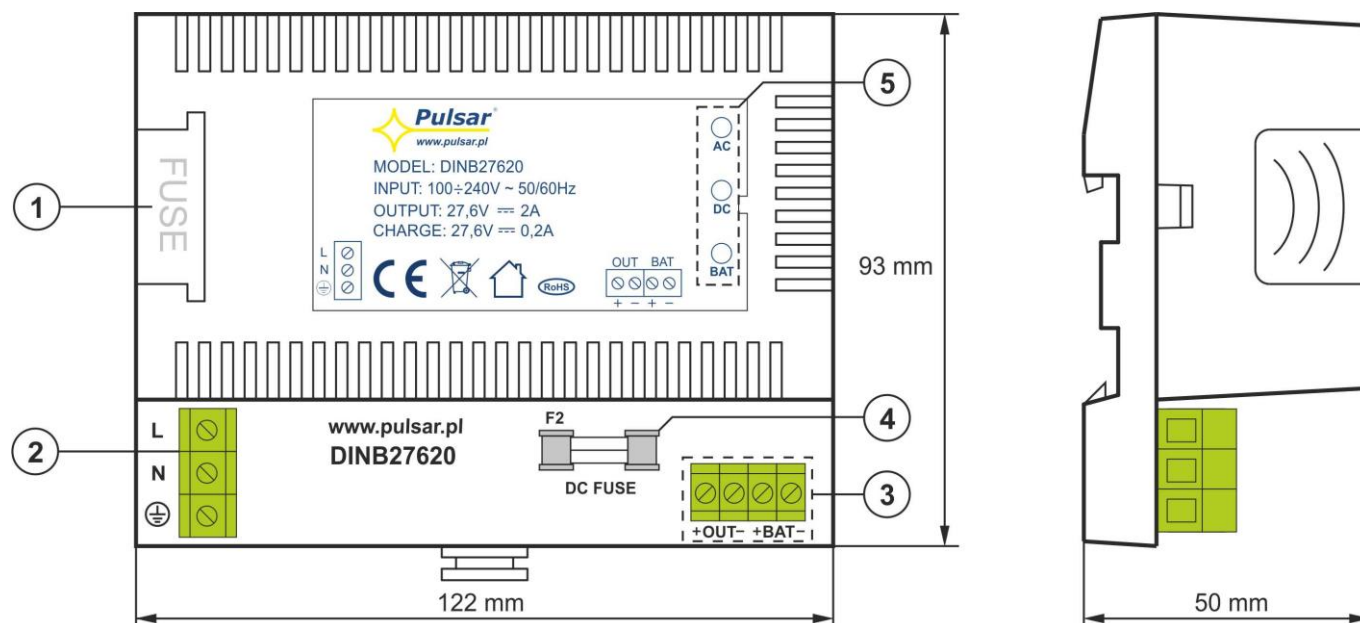
Fig. 2. The view of the PSU module.
