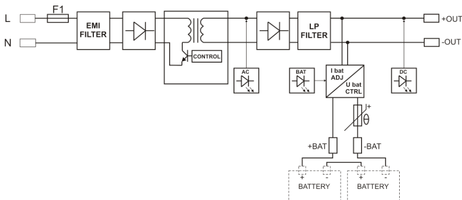
Fig.1. Block diagram of the PSU.
