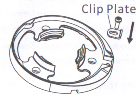
Figure 2-5 Screw the Clip Plate
