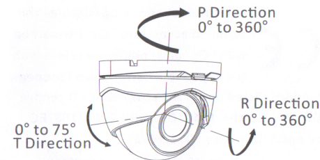
Figure 2-7 3-axis Adjustment
