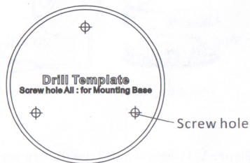
Figure 2-1 The Drill Template
