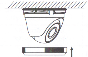
Figure 2-10 Fix the Trim Ring to the Camera
