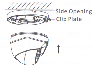
Figure 2-6 Fix the the Camera
