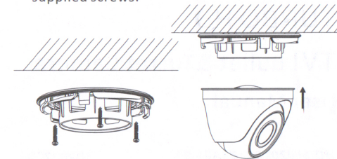
Figure 2-9 Fix the Mounting Base and Camera
