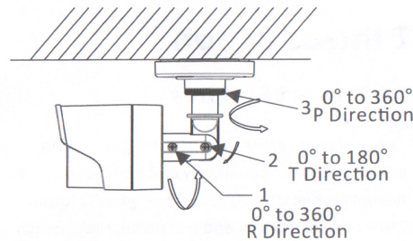
Figure 2-3 3-axis Adjustment
