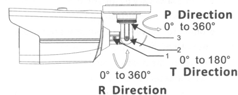
Figure 2-3 3-axis Adjustment
