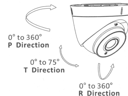
Figure 2-6 3-axis Adjustment
