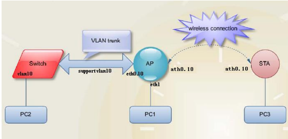
Figure 7-32 VLAN Settings
