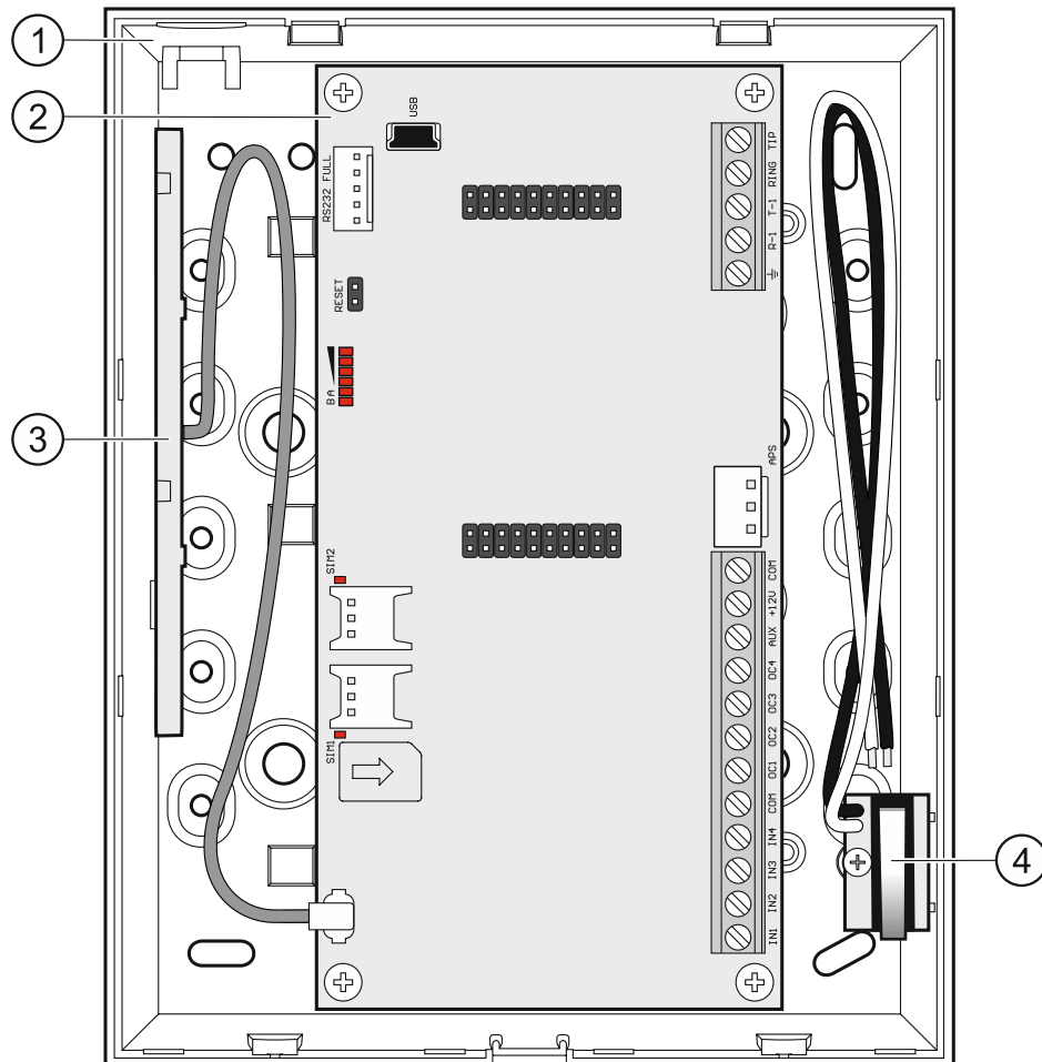
Fig. 2. GSM-X module in OPU-2B enclosure.
