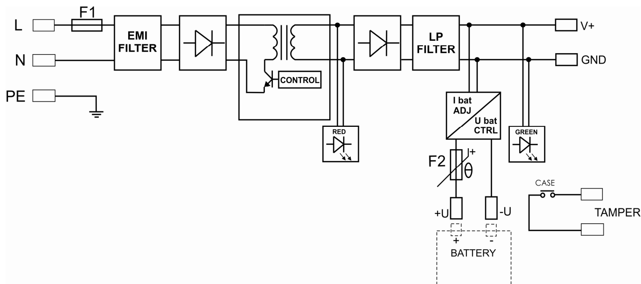
1.2 Block diagram Fig.1
