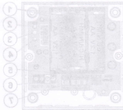
Figure 1: 1 – rechargeable batteries; 2 – DOOR output indicator; 3 – JA-100 BUS activity indicator; 4 – IN input activation indicator; 5 – LEARN (tamper) tamper contact; 6 – BUS terminal; 7 – input and output terminals (NO)
