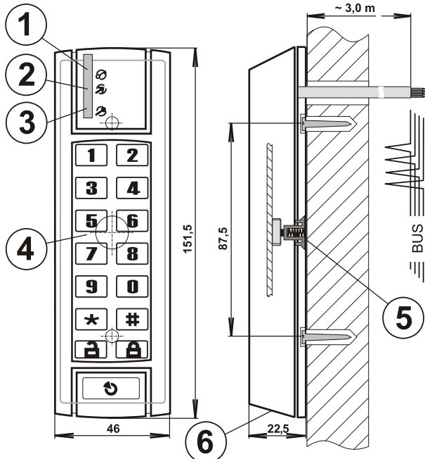
Fig.: 1 – red LED indicates an armed (set) section, 2 – green LED indicates a disarmed (unset) section, 3 – yellow LED indicates fault/service mode, 4 – keypad and reading area, 5 – tamper contact; 6 – screw for holding the plastic cover
