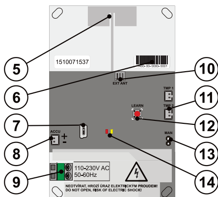
Figure 3: 5 – antenna; 6 – production code; 7 – miniUSB connector 8 – backup battery connector; 9 – mains terminals and protective foil; 10 – external antenna connector; 11 – tamper contact connectors; 12 – LEARN button; 13 – MAN terminal for manual boot from powered backup battery; 14 – LED indicators
