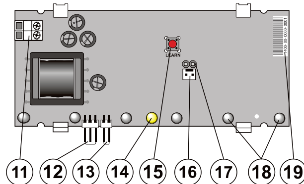
Fig. 2: 11 – 12V DC power terminals; 12 – piezo siren connection (attention: high voltage); 13 – backup battery connection; 14 – yellow fault indicator; 15 – LEARN (enrolment) button; 16 – external antenna connection; 17 – external antenna jumper; 18 – high intensity red LED flashers; 19 – production code
