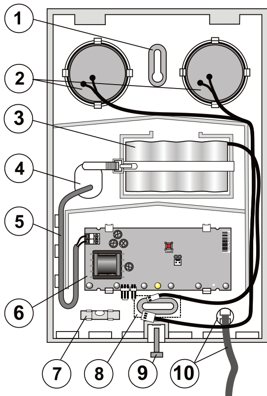
Fig. 1 – hole for installing; 2 – piezo sounders; 3 – NiCd battery with reusable battery strap; 4 – hole for cable; 5 – 12V DC power cable; 6 – PCB; 7 – spirit level; 8 – hole for installation with tamper detection; 9 – front cover screw; 10 – string with clip connecting the front cover for easy installation
