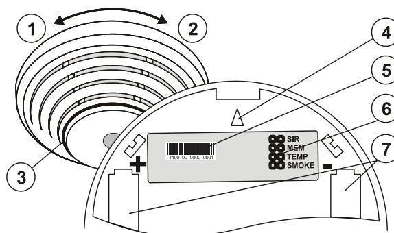
Fig 1: 1– detector cover opening; 2 – detector cover closing; 3 – optical status signalling; 4 – arrow showing where to insert the detector; 5 – production code; 6 – configuration terminals; 7 – battery holders
