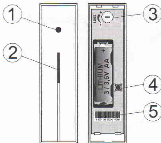
Figure: 1 – sound sensor; 2 – red LED activation indicator; 3 – trimmer for pressure sensitivity adjusting; 4 – tamper contact; 5 – production code
