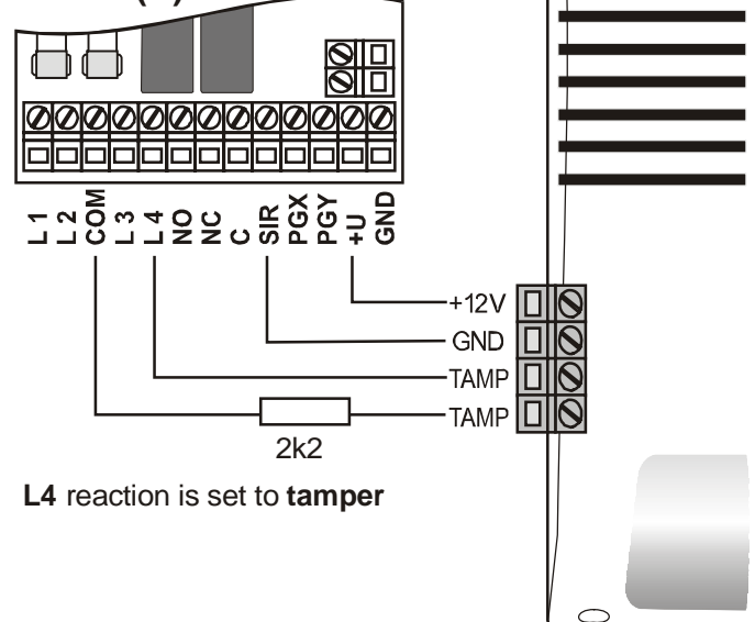
Picture 2 - example of connection with the JA-63K(R) control panel
