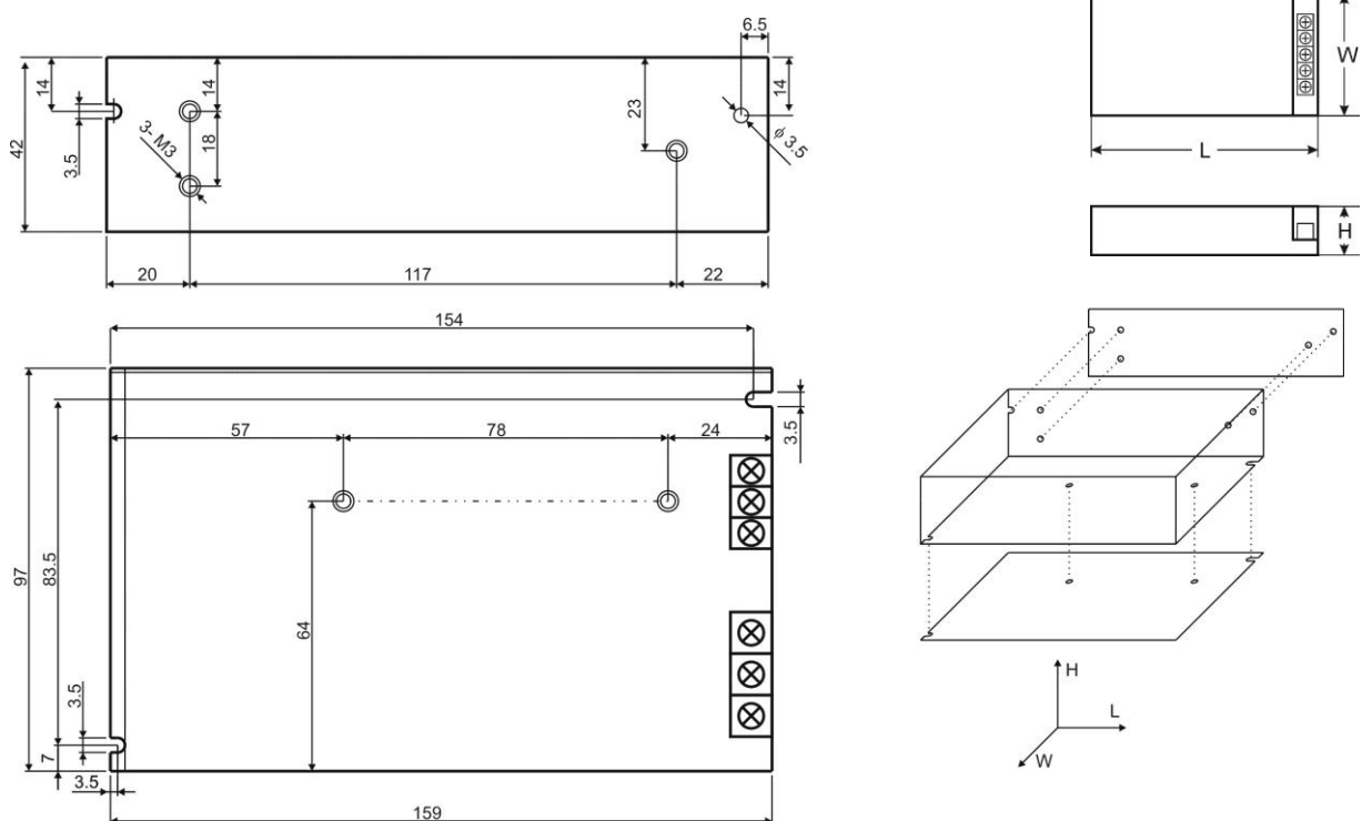
Fig. 2. Dimensions of power supply.
