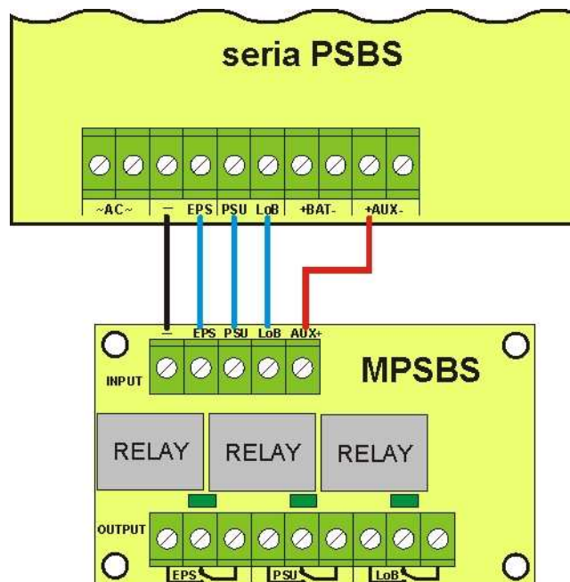
Fig. 5. The diagram of connecting the MPSBS module.
