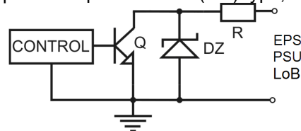
Fig. 4. Electrical diagram of the OC technical outputs.
