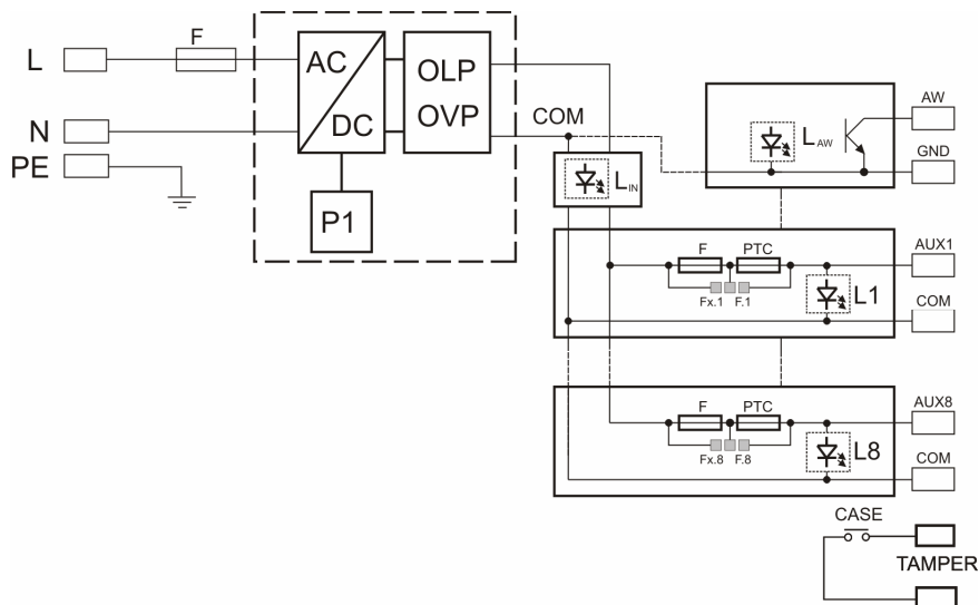
Fig.1. Block diagram of the PSU.
