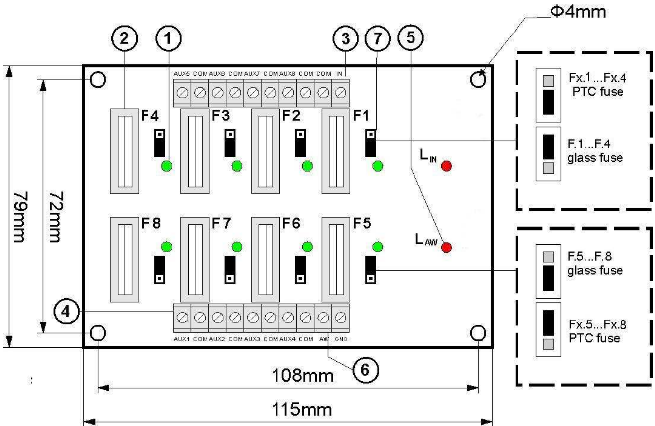
Fig.2. The view of the PSU's pcb.
