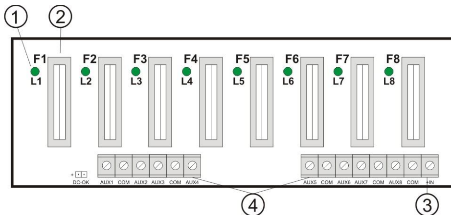
Fig.2. The view of the PSU's pcb.
