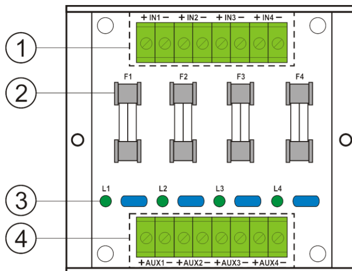
Fig.2. The view of the PSU's pcb.
