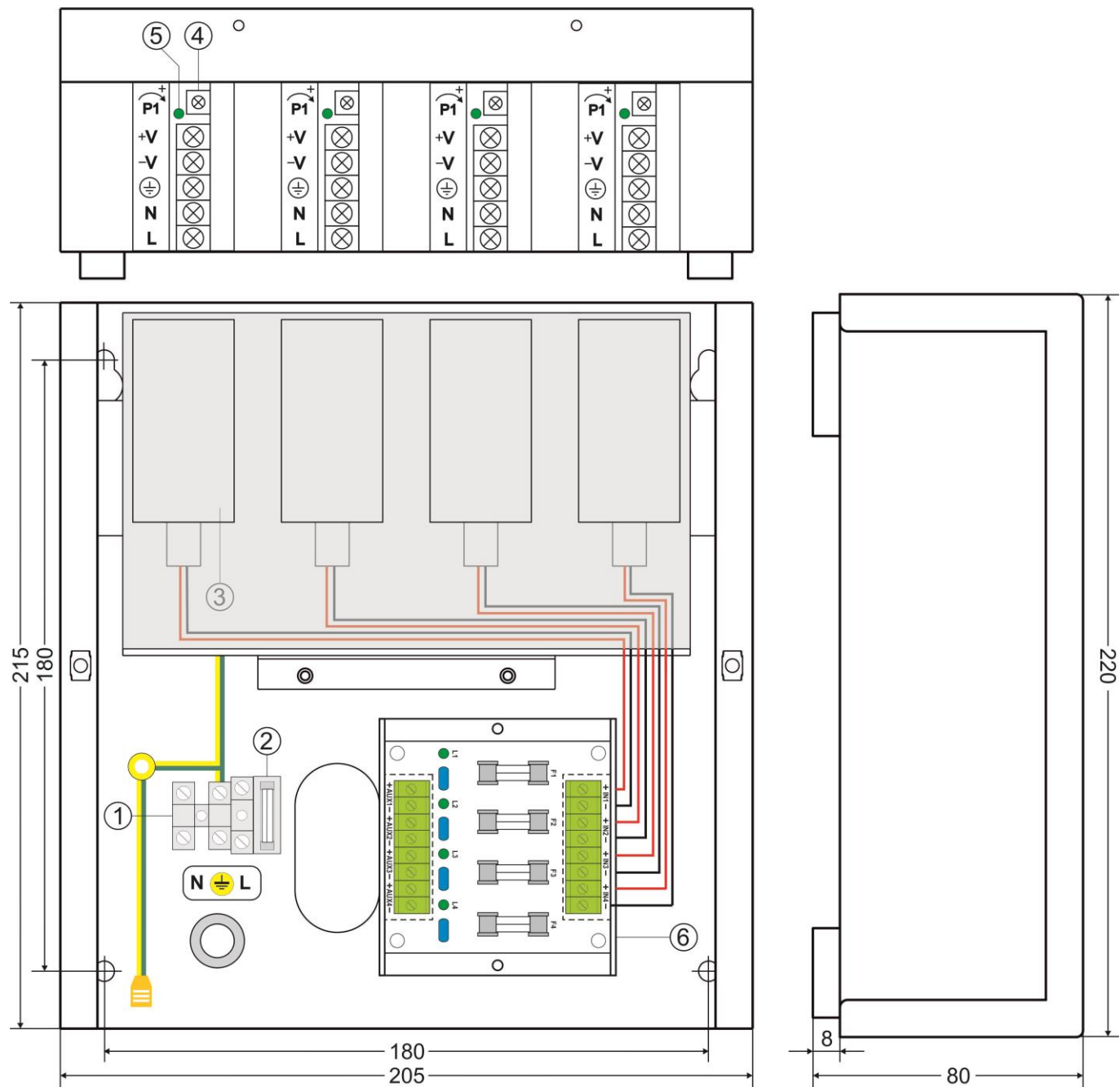
Fig.3. The view of the PSU.
