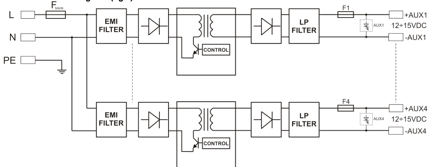
Fig.1. Block diagram of the PSU.
