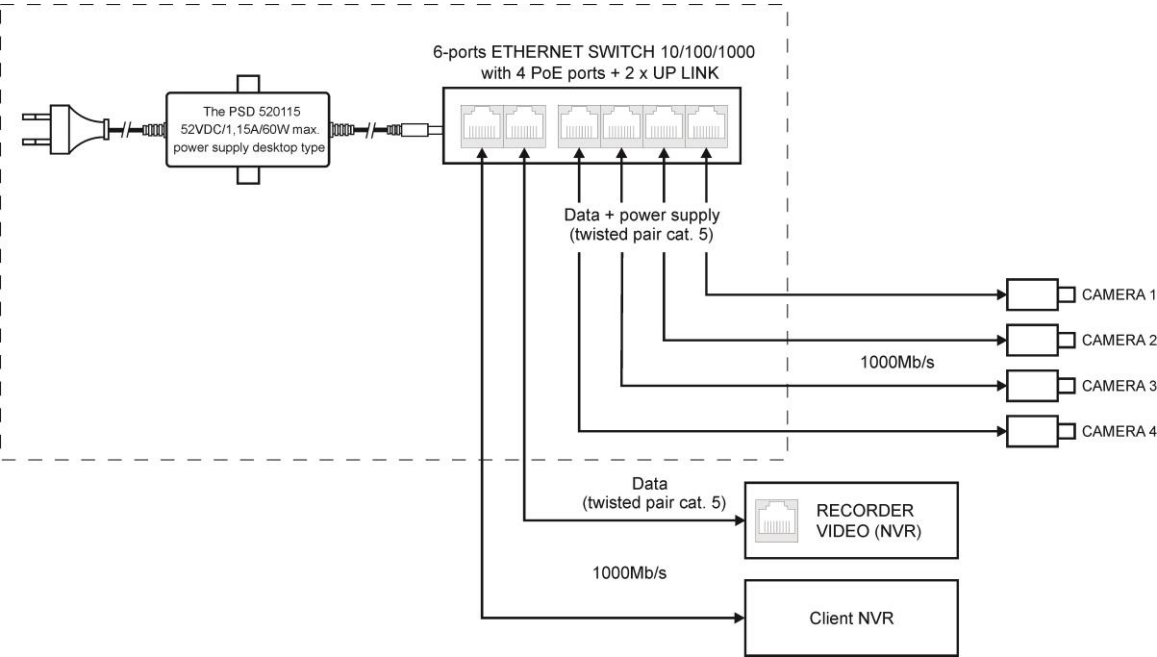
Fig. 1. Block diagram.
