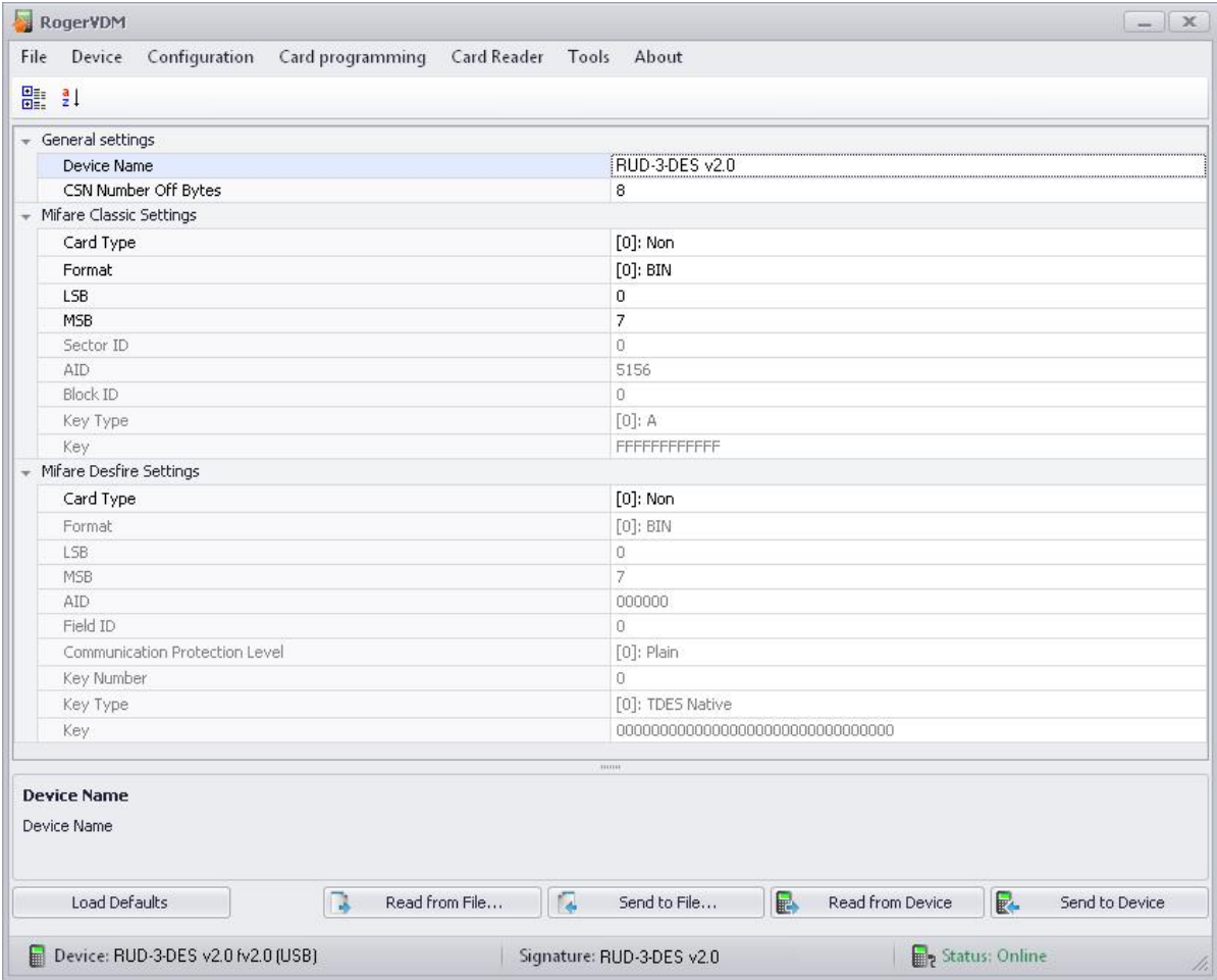
Fig.6 Device configuration window.
