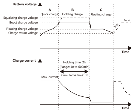
Figure 1-5 Battery charging stages curve graph
