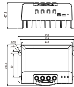
Model : MC2430N10 ; Outline dimensions : 150*105.6*67.5mm ; Mounting dimensions : 139*60mm ; Fixed holes dia : \Phi 5mm ; Wire specifications : 20-6AWG.
