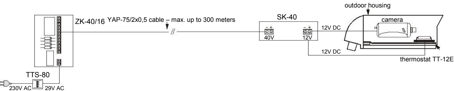
Schematic diagram for one camera with thermostat:
